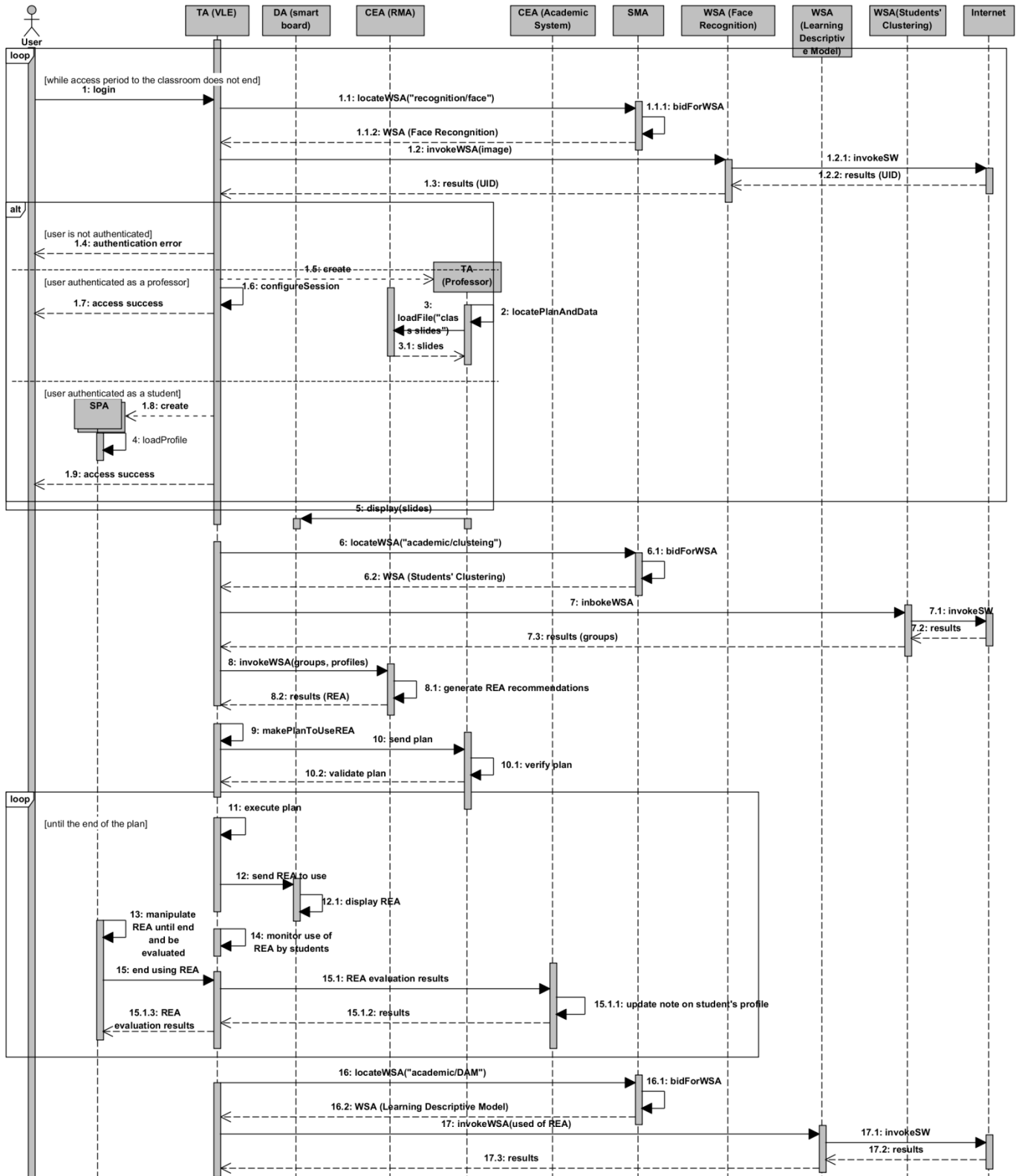
Figure 5. Conversation "online tutoring process"
