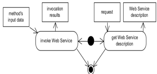
Figure 4. Activities Diagram for the "Invoke Web Service" Use Case.
