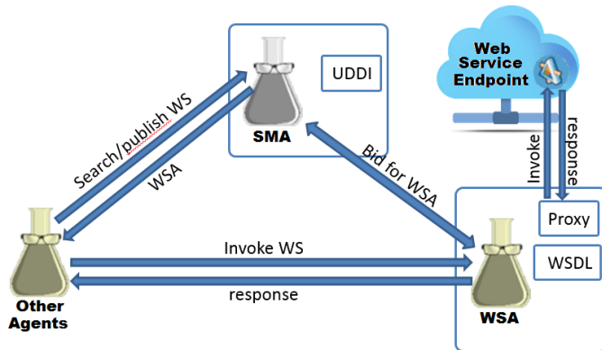
Figure 2. Agents and Cloud Services Integration.
