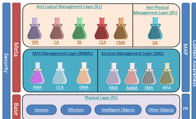
Figure 1. AmICL Proposed architecture.
